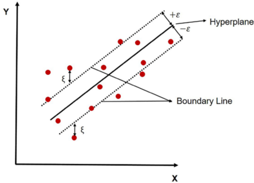
Figure3. Graphical representation of support vector regression
