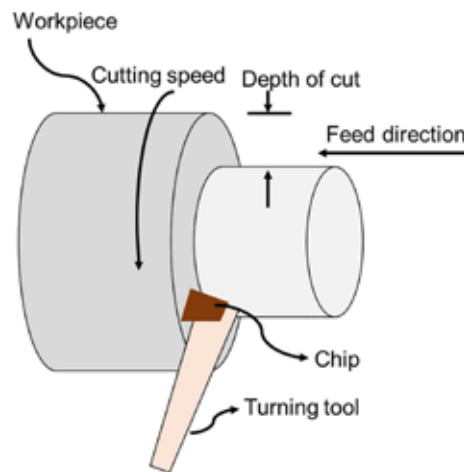
Figure1. Machining of turning operation
